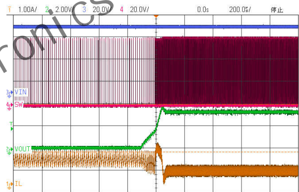
(22) Short Output Recovery (VIN=60.0V, OUT=3.3V, IOUT=0.6A)
