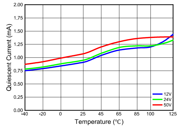
(11) Quiescent Current VS Temperature
