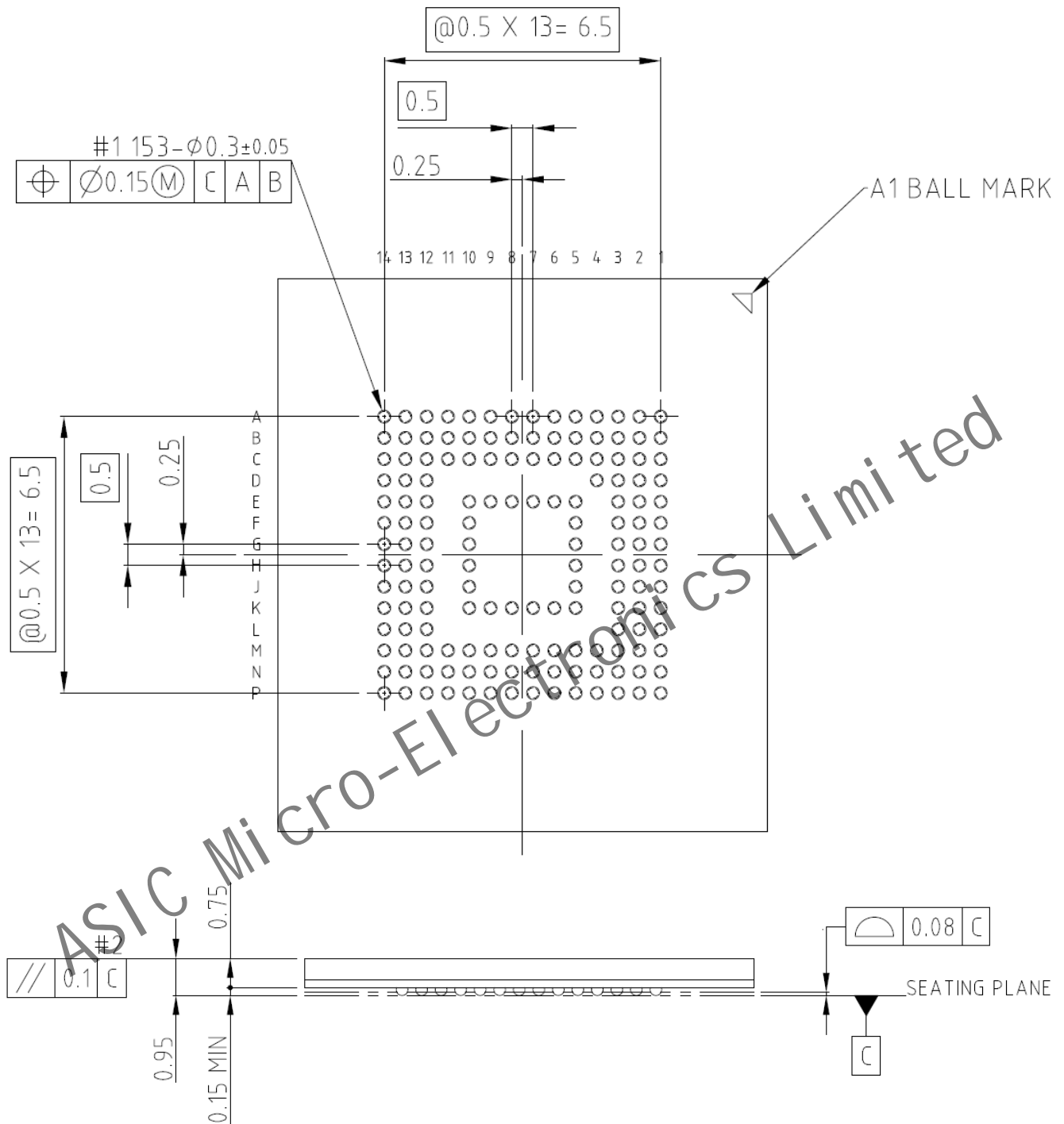
Figure 5 – 11.5 x 13.0 x 1.0mm Bottom & side View
