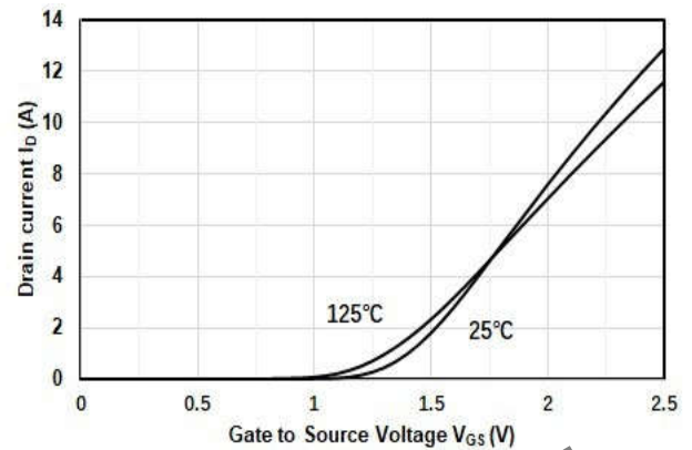
Transfer Characteristics
