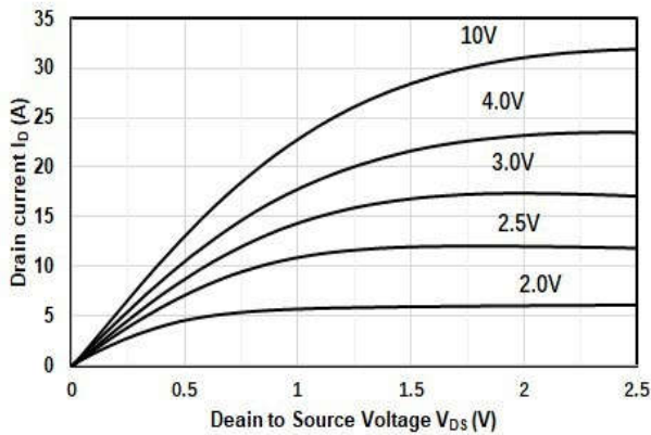
Output Characteristics
