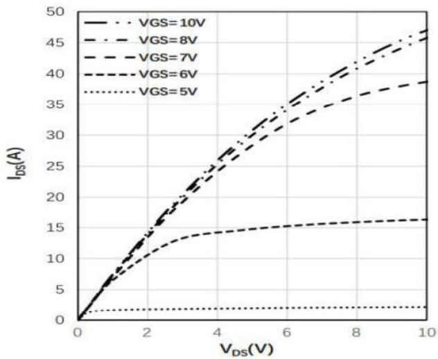
Fig.1 Typical Output Characteristics ( 25^{\circ}\text{C} )
