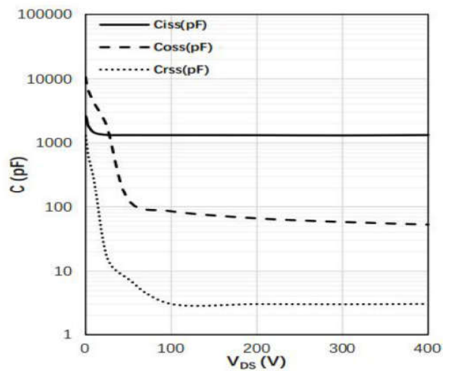
Fig.6 Typical Capacitance
