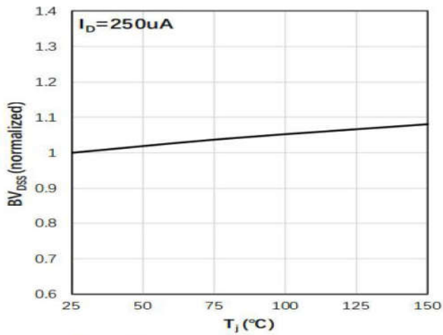
Fig.7 Breakdown Voltage vs. Temperature Characteristic
