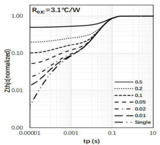
Fig.12 Transient Thermal Impedance
