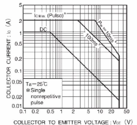
Fig.9 Safe operating area
